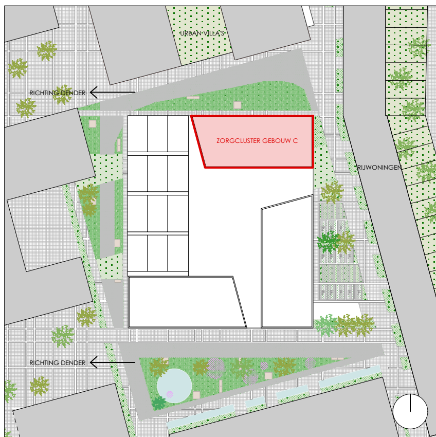
INPLANTINGSPLAN
