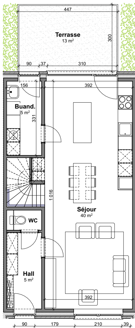
Rez
