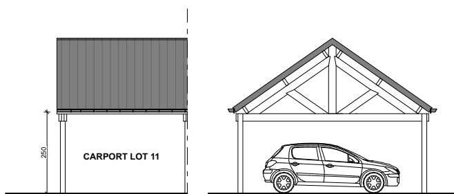
Façades Car-port
