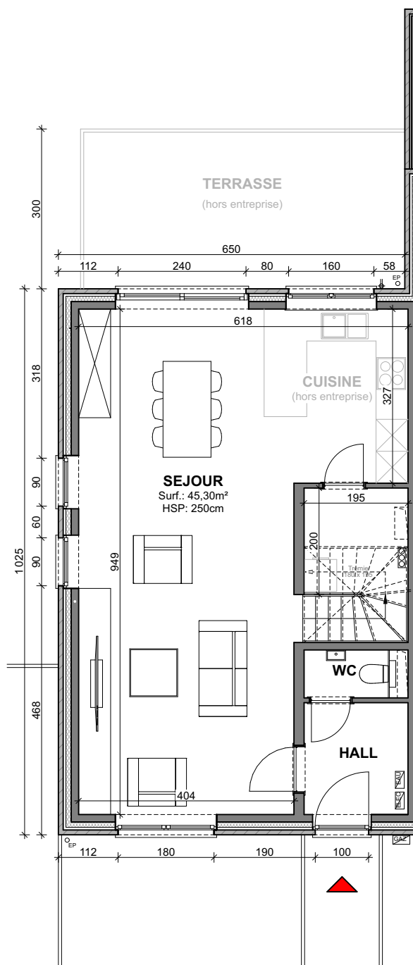
Plan - Rez
