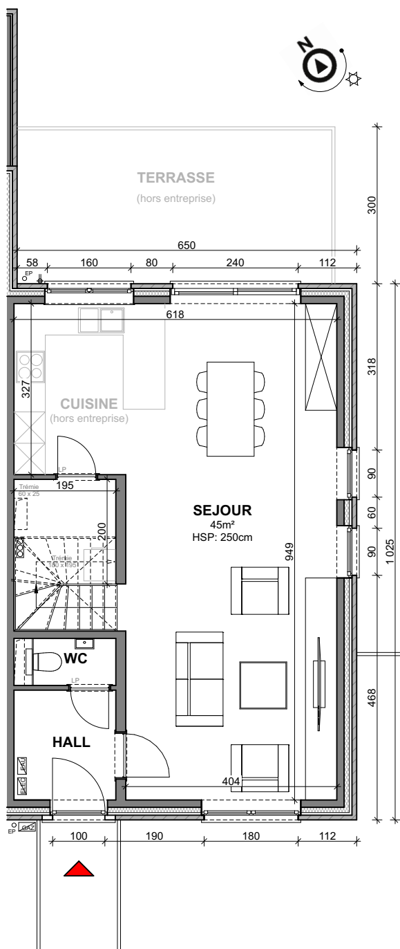
Plan - Rez
