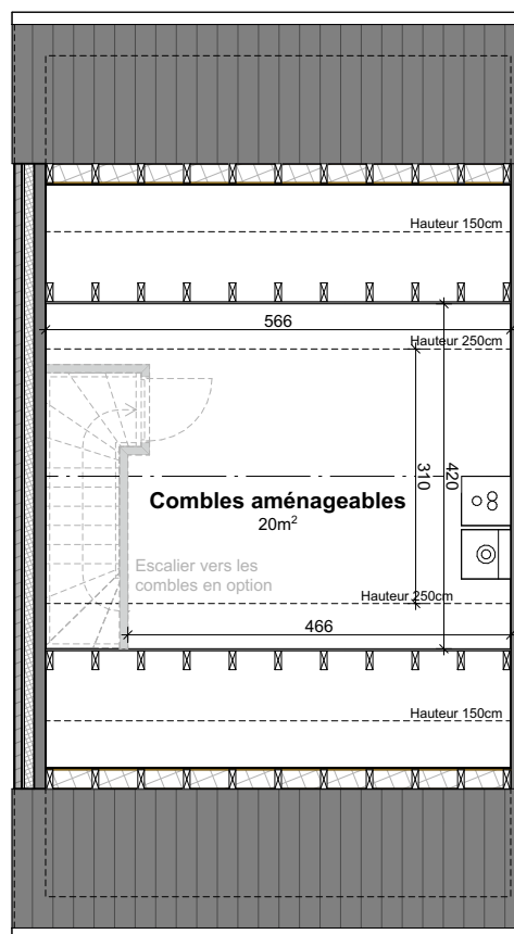
Combles
