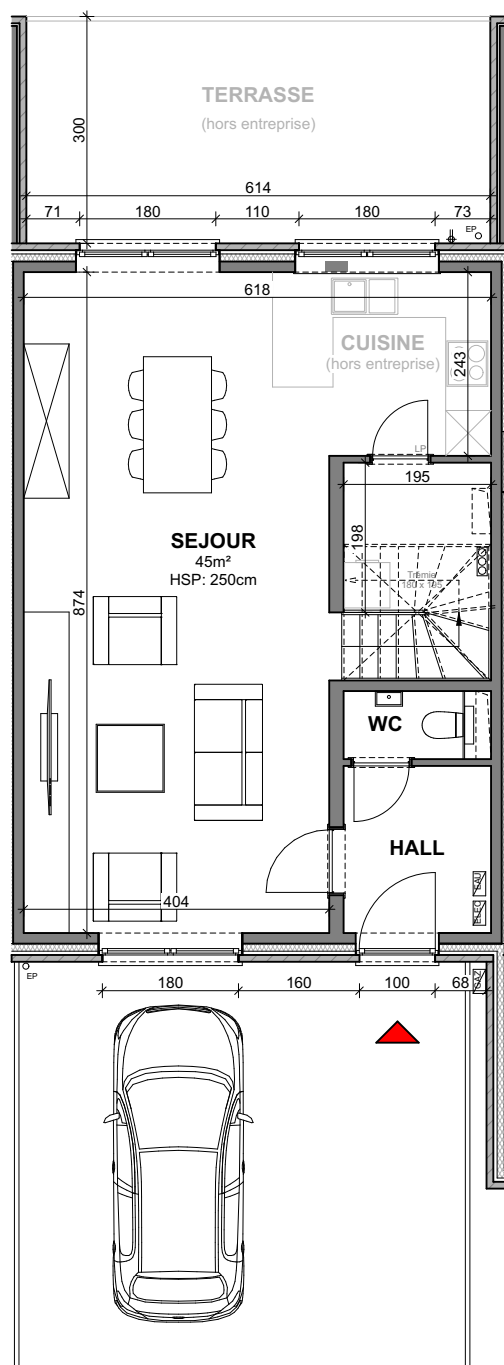
Plan - Rez
